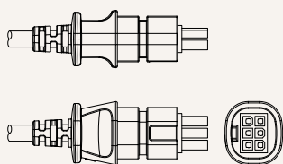
R = Molex 6P, 180° plug
