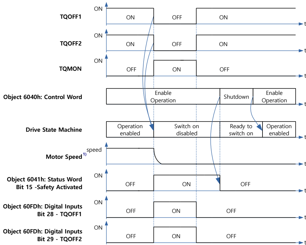
Figure 4.16: Safety Function Timing Chart
