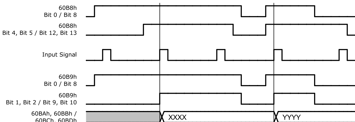
Figure 4.12: Touch Probe Operation (Bit 1 / Bit 9 = 0)
