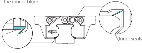
Bottom Seals
